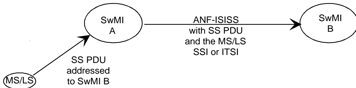
Figure 1: SS PDU addressed by a MS/LS to a distant SwMI
